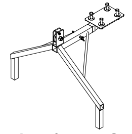
Winch/Pulley Stand TRS-WPS Overall Length 38"
