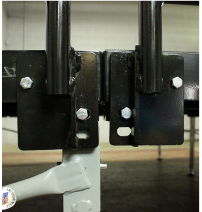
Closeup of guardrail attached to stage decks.
