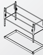
INDY-GRT6 Guard Rail Package (Includes toeboard)
