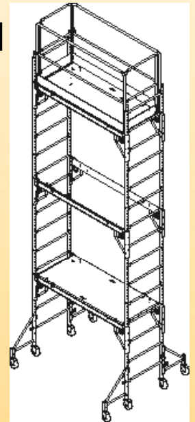
SP-6TR Wt. 523# 17'H x 6'L x 29"W Triple Unit Consists of 2 single units, one 65" add unit, one guard rail set, and 4 wide outriggers
