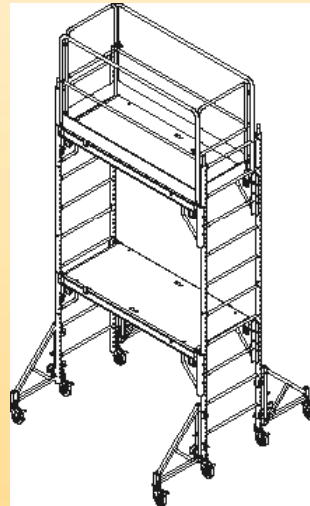
SP-6D Wt. 386# 12'H x 6'L x 29"W Double Unit Consists of 2 single units, one guard rail set, and 4 narrow outriggers.
