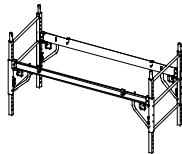
SP-8AD3 39" Add-on unit
